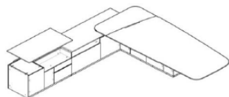
HORI-3131-B-L/R W3150 x D3120 x 750H MAIN DESK: W2800 x D1200/1000 x H750 SIDE CABINET: W2800 x D600 x H640mm ADJ. TABLE: W1170 x D600 x H640mm
