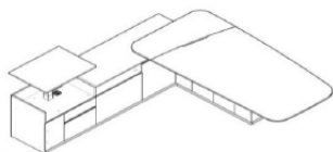
HORI-2728-B-L/R W2750 x D2720 x 750H MAIN DESK: W2400 x D1200/1000 x H750 SIDE CABINET: W2400 x D600 x H640mm ADJ. TABLE: W800 x D600 x H640mm
