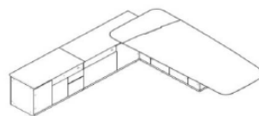
HORI-3131-A-L/R W3150 x D3120 x 750H MAIN DESK: W2800 x D1200/1000 x H750 SIDE CABINET: W2800 x D600 x H640mm
